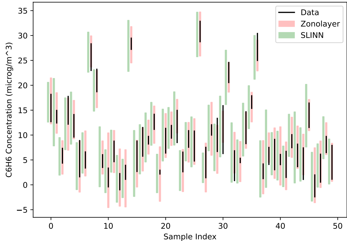
Air Quality Dataset — Benzene Concentration
